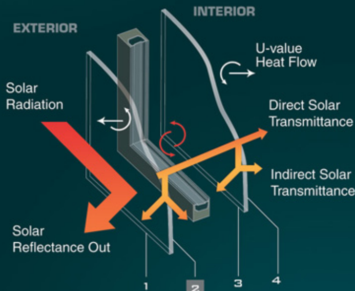
SOLAR HEAT GAIN DIAGRAM
